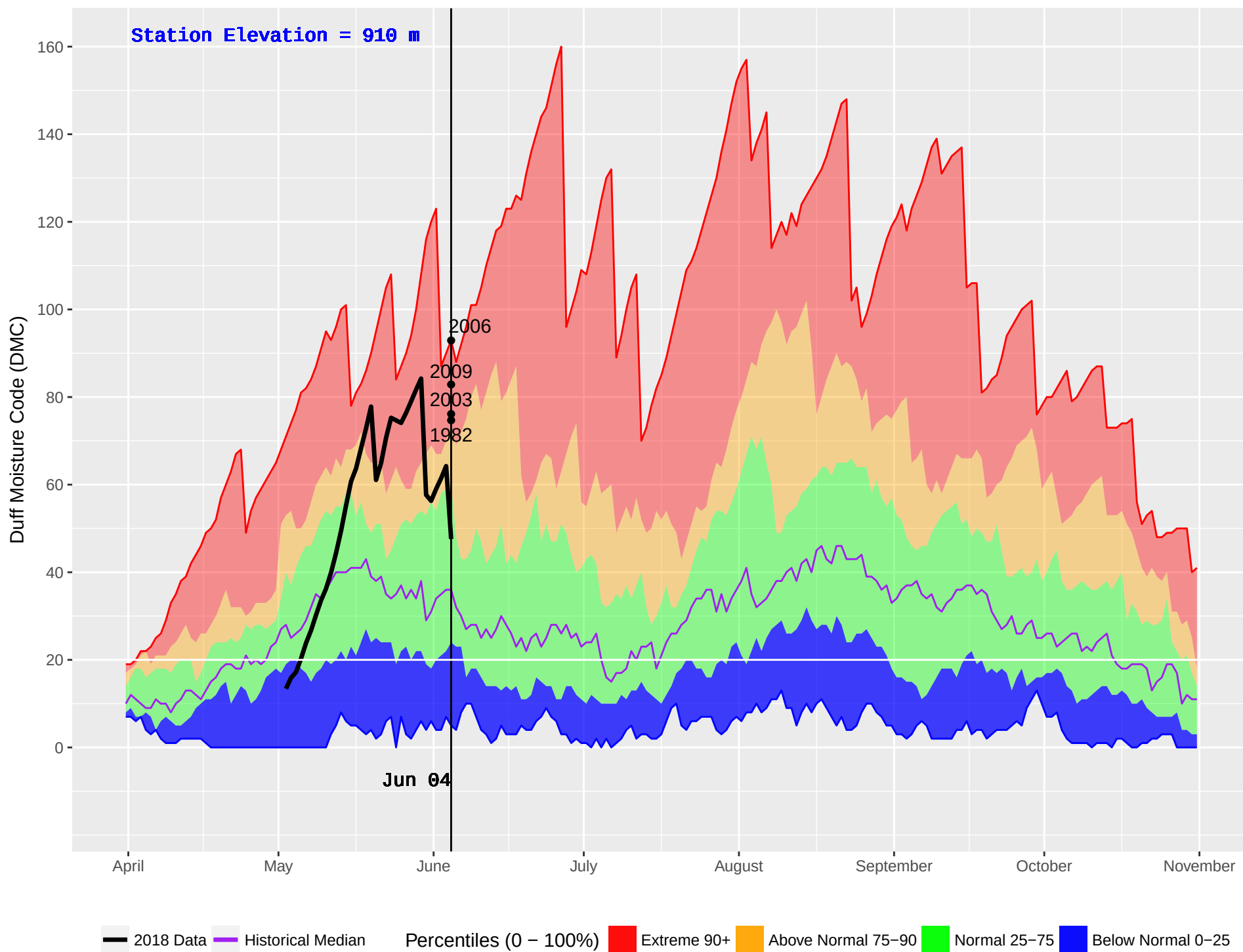
NAZKO (211) : Historical (1981–2016) and Current (2018) Noon Duff Moisture Code (DMC)
